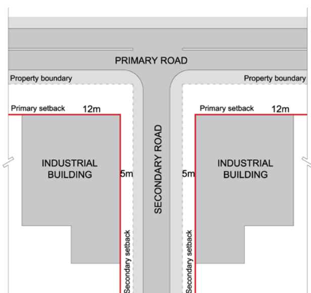
Figure 18. Corner site setbacks
