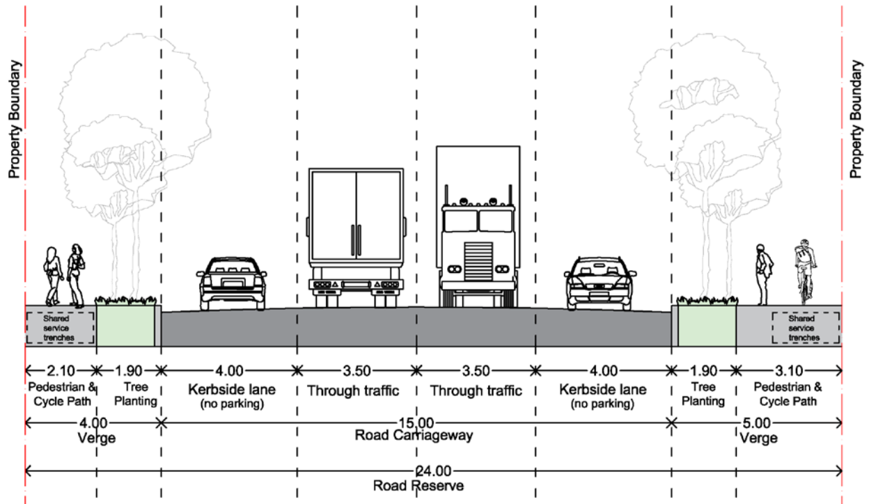
Figure 13. Typical Local Industrial Road (Type 1)
